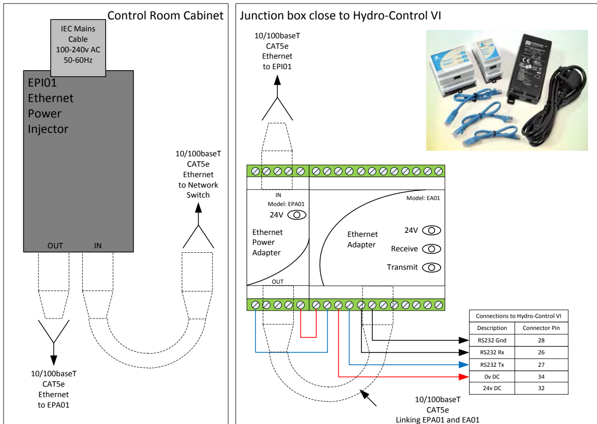
Figure 6: Connecting the Ethernet Adapter to Hydro-Control VI with Power Over Ethernet Option
