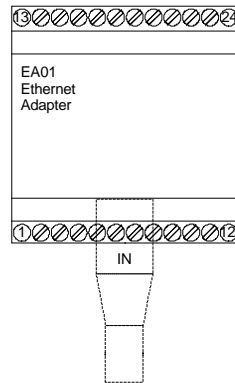
Figure 7: EA01 Terminal Identification
