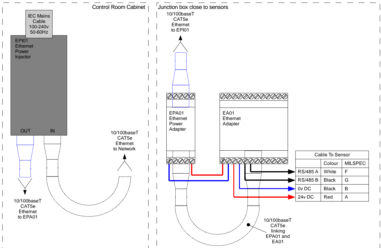
Figure 3: Connections for Ethernet Adapter and Power Adapter
