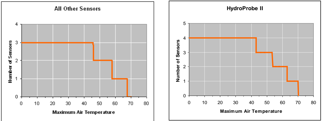
Figure 4: Maximum number of sensor connections dependent upon ambient temperature
