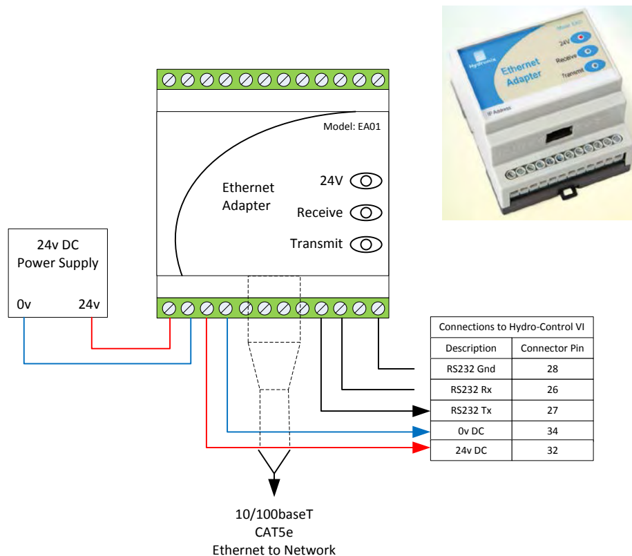
Figure 5: Connecting the Ethernet Adapter to Hydro-Control VI
