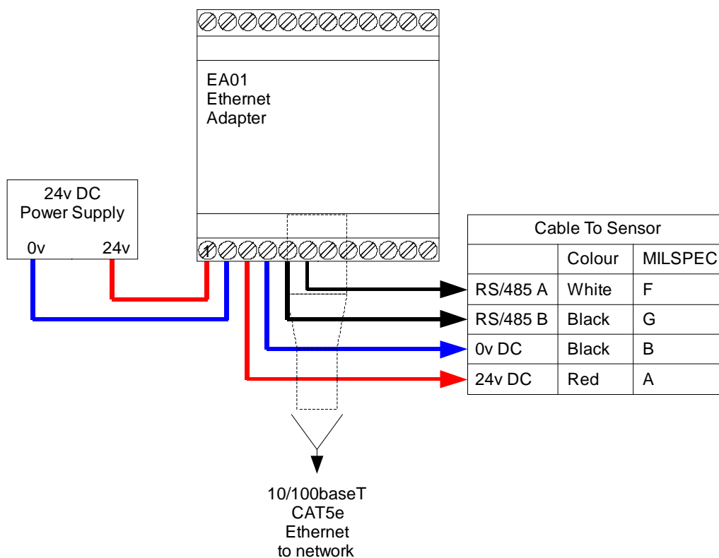
Figure 2: Connections for Ethernet Adapter only
